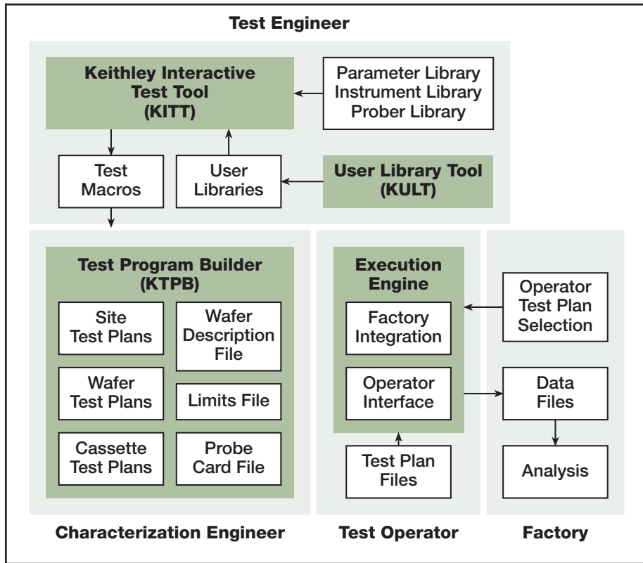
Figure 3. KTE software architecture
