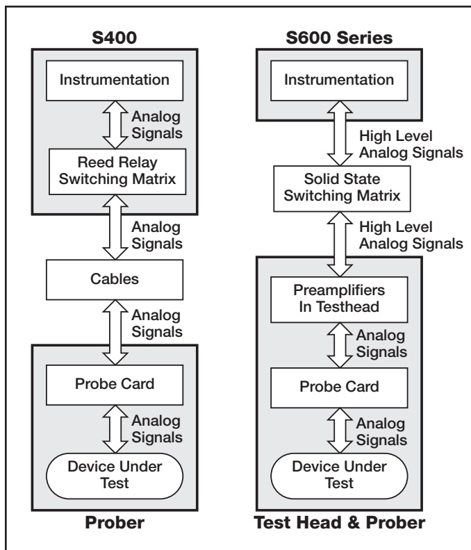
Figure 2. Comparison of the “per-pin electronics” architecture of S600 Series systems to the “cabled-out” design of S400UX systems. The S600 Series architecture improves current sensitivity by minimizing the parasitic capacitances and leakage currents inherent in systems with long cables and a reed-relay-based switch matrix between the DUT and the measurement circuitry.
