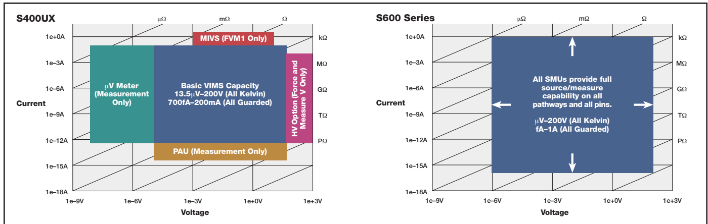
Figure 1. S400UX and S600 Series measurement ranges
