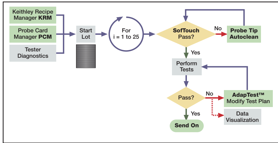
Figure 4. Keithley can provide a complete operational model for a parametric test cell.
